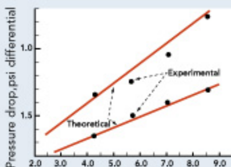
Flux density lbs/hr/ft 2 X 10 3 a. MIL-H-5606 hydraulic oil at 100°F
