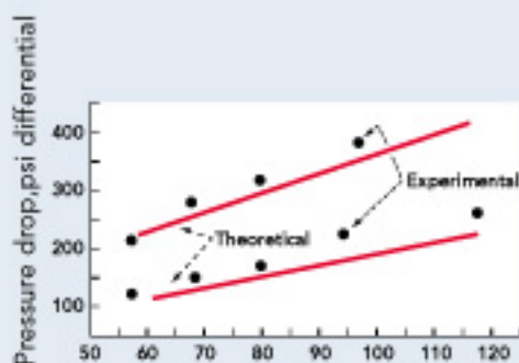
Flux density lbs/hr/ft 2 b. VFR5620A polyester at 290°C
