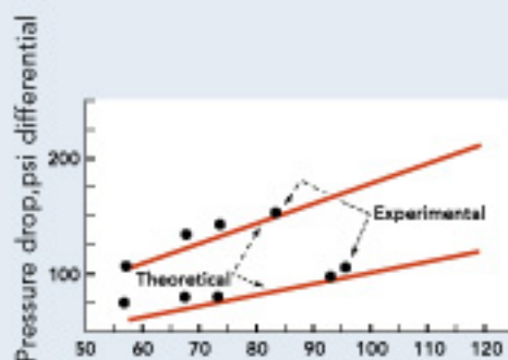
Flux density lbs/hr/ft 2 b. VFR5442C polyester at 290°C
